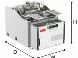
ACS880-304LC, D8T
